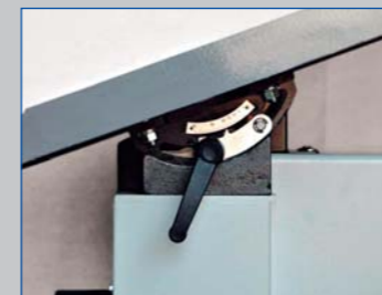
Piano inclinabile 20° 20° tilting table Table inclinable de 20° 20° schrägstellbarer Tisch Mesa inclinable 20°
